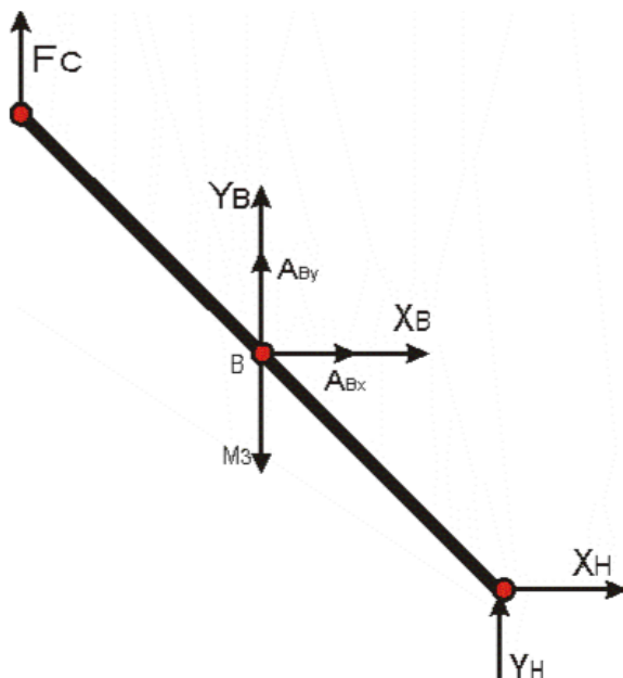
Fig. 6. Linkage I–Equilibrium conditions for the point CH
