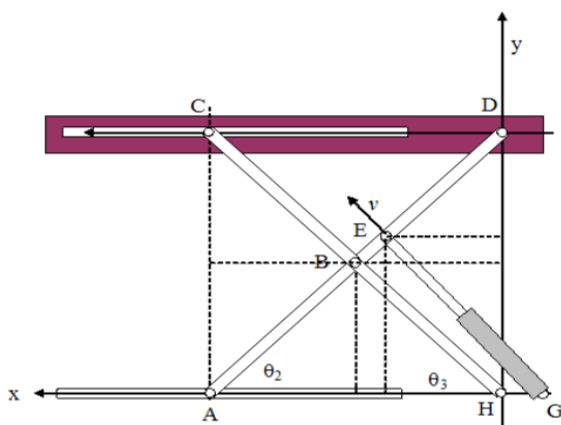
Fig. 1: Linkage ADH, and crank mechanism ACH
