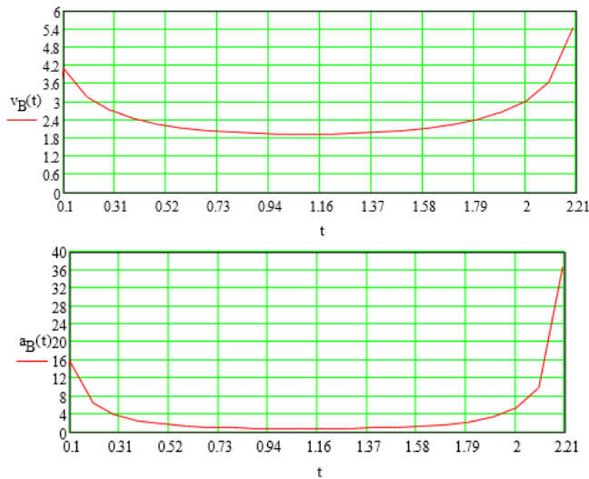
Fig. 4 Velocities and acceleration of point B
