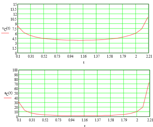
Fig. 3 Velocities and acceleration of point C
