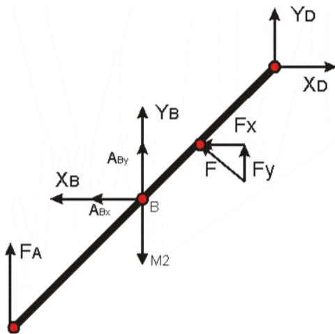
Fig. 5 Linkage I–Equilibrium conditions for the point AD
